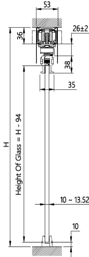
Type 2: Frameless (SDS-100GC-BK)
