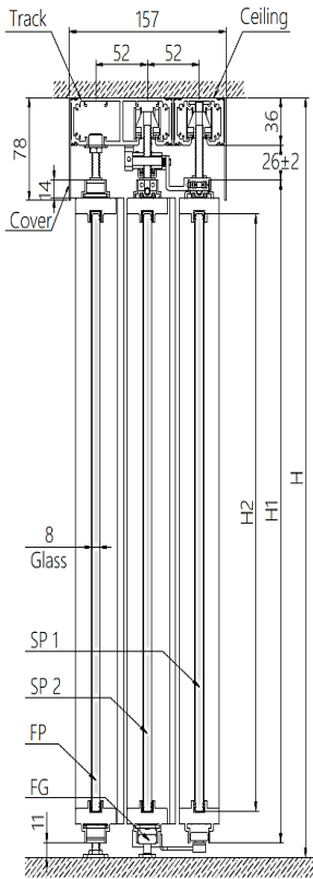
Type 1: Ultra Slim (2S+1F)
