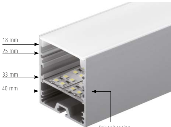
Driver housing code ZK73100-SL
