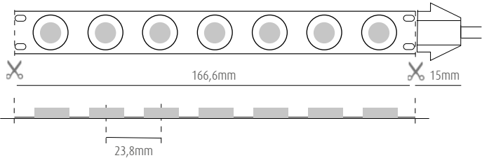
LED SPACING AND PITCH CUT
