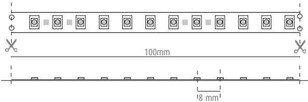
LED SPACING AND PITCH CUT
