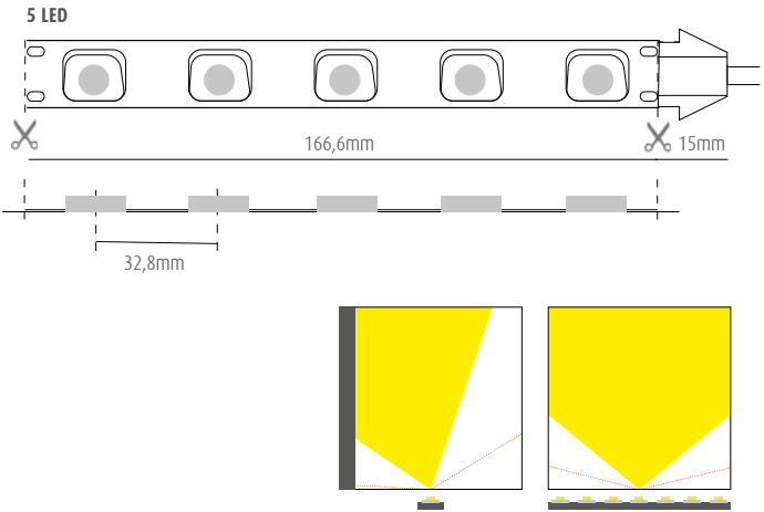
LED SPACING AND PITCH CUT
