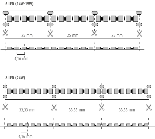
LED SPACING AND PITCH CUT
