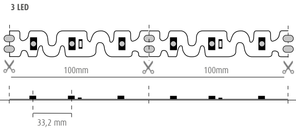
LED SPACING AND PITCH CUT
