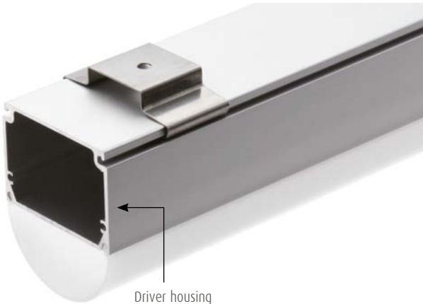
Driver housing code ZK73100-SL
