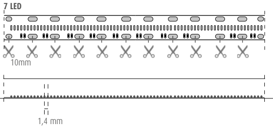
LED SPACING AND PITCH CUT
