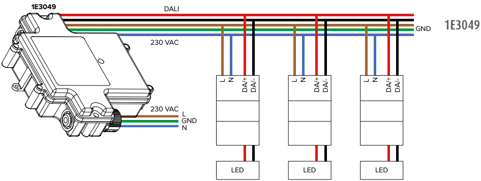
DALI MULTIPLE CONTROL IP67
