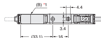
Mounting Holes
