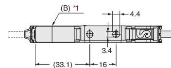
Mounting Holes
