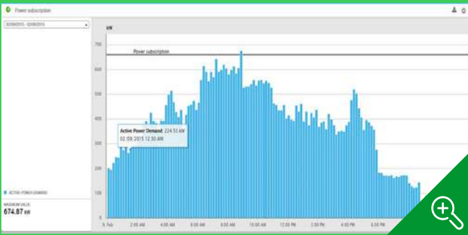
Power demand with target
