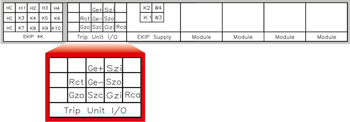
25) Transformer star center (homopolar) current sensor input
