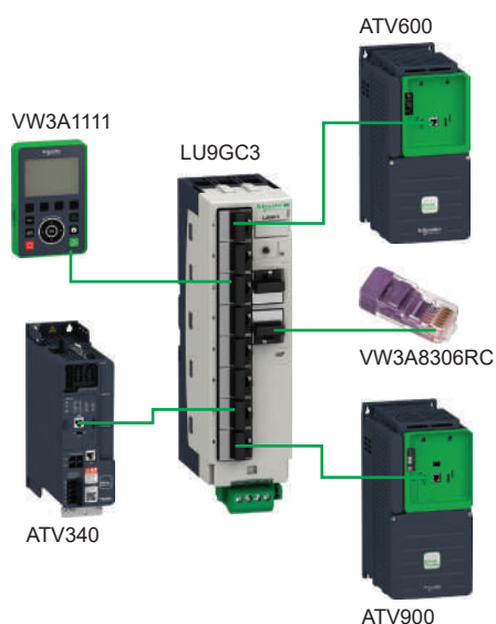
Example of multipoint screen architecture
