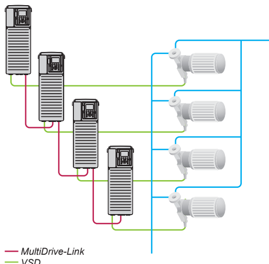
Example of connection with MD-Link
