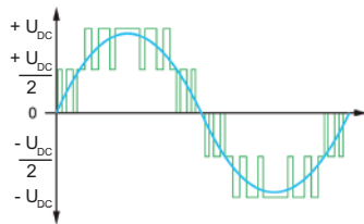
ATV600 with 3-level technology
