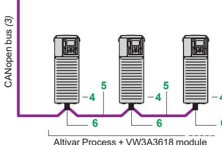
Example of connection to the CANopen bus via SUB-D connector
