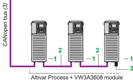
Optimized solution for daisy chain connection to the CANopen bus
