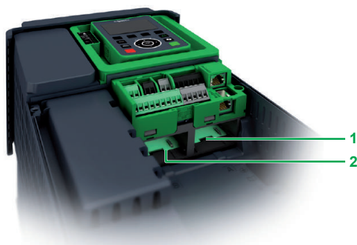
Altivar Process drives slots for additional I/O modules
