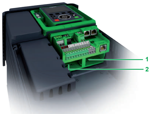
Altivar Process drives slots for additional I/O modules
