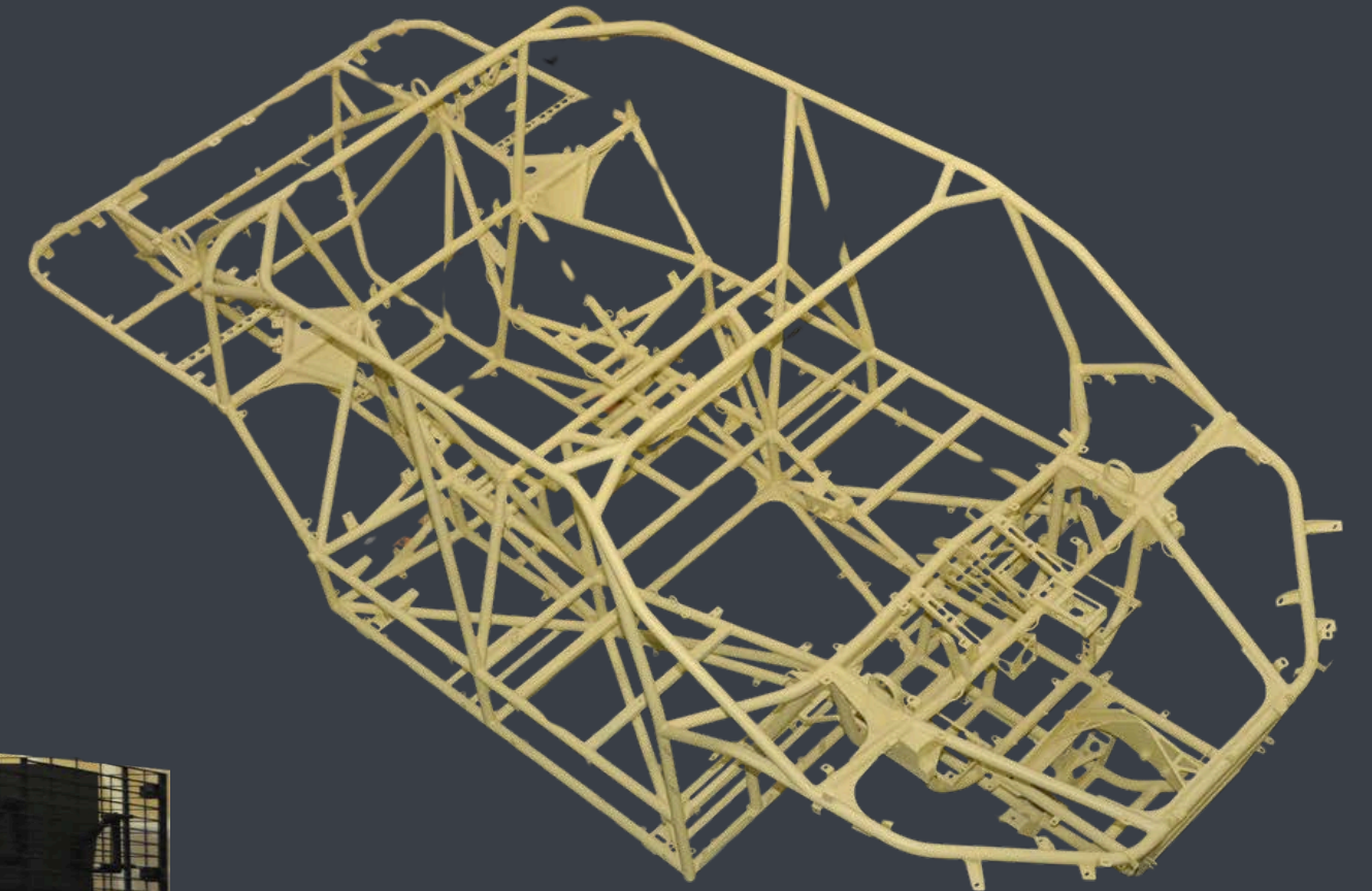
STEEL PIPE VEHICLE CHASIS
